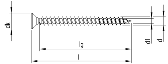
Dimension Drawing
